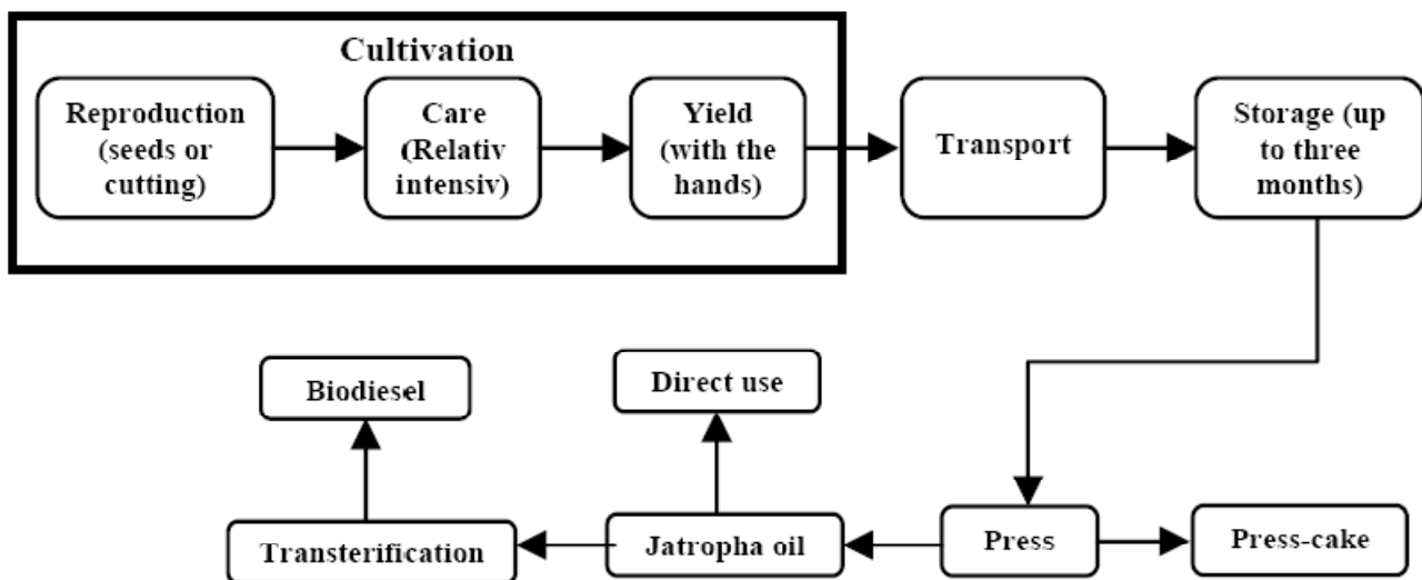
Fig. 2. General process chain for the biodiesel production from Jatropha curcas
